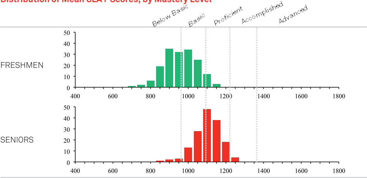
Distribution of Mean CLA+ Scores, by Mastery Level
